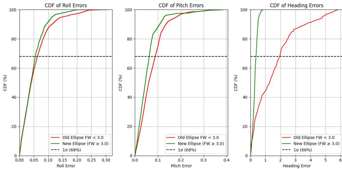
Figure 6: CDF of the roll and pitch errors
