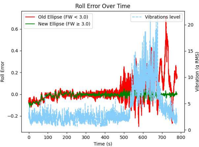
Figure 8: Roll error over time
