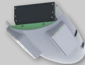
Synthetic-aperture radar (SAR) 2
