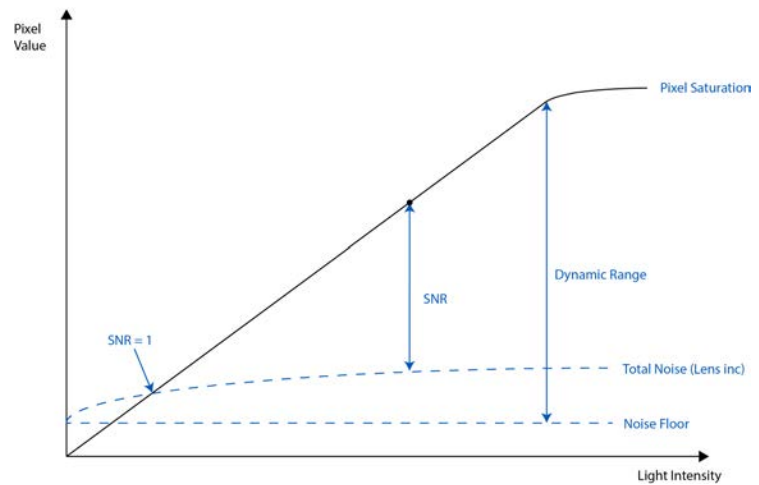
Figure 4 – Illustration of SNR and DR with Respect to Pixel Value vs Light Intensity
