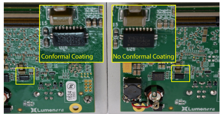
Figure 5 – Comparing two identical circuit boards - one with conformal coating, one without
