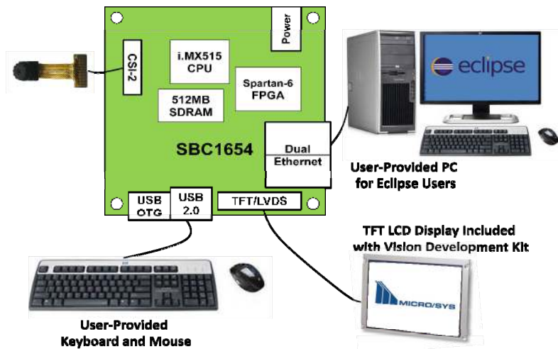
SBC1654 Development Platform Setup
